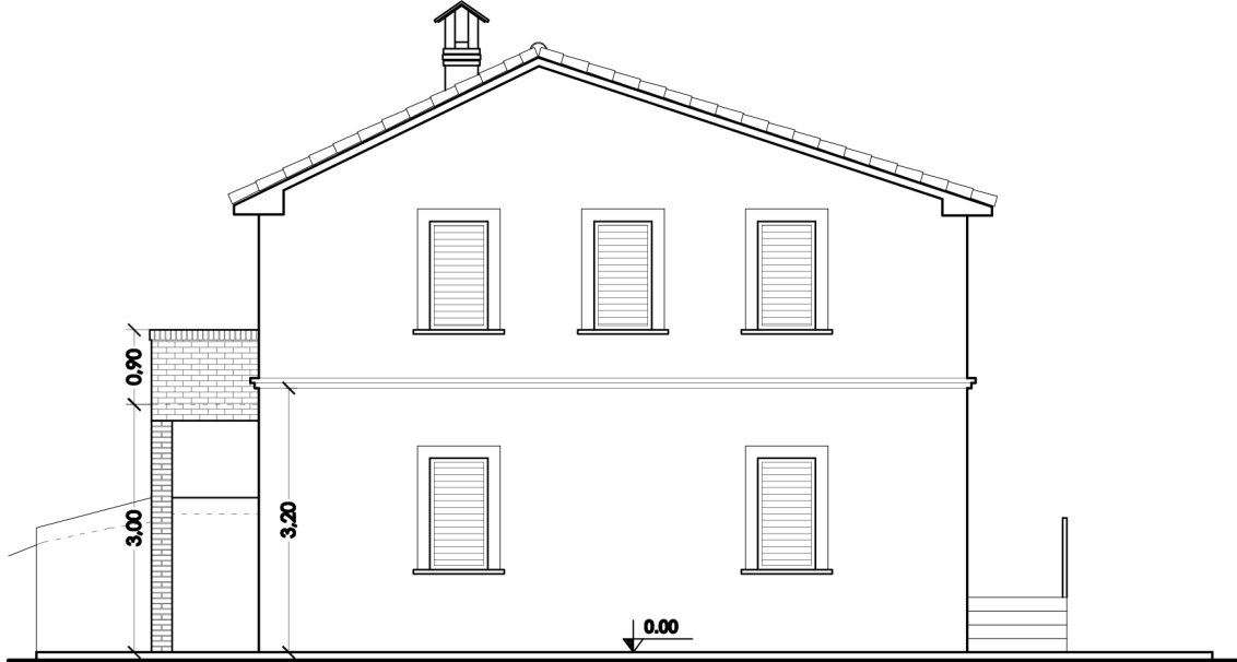
SOUTH VIEW
