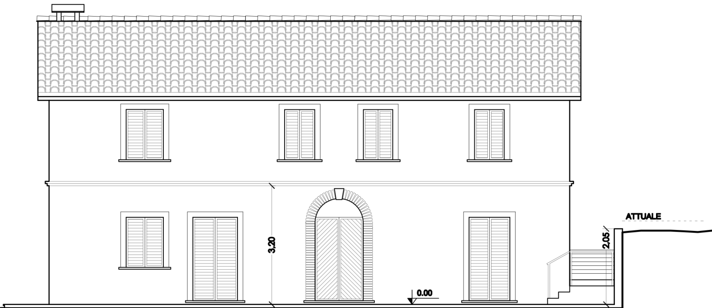
EAST VIEW
