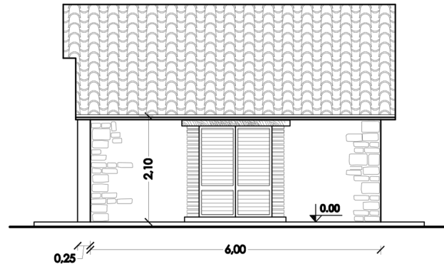
EAST VIEW Scale 1:100
