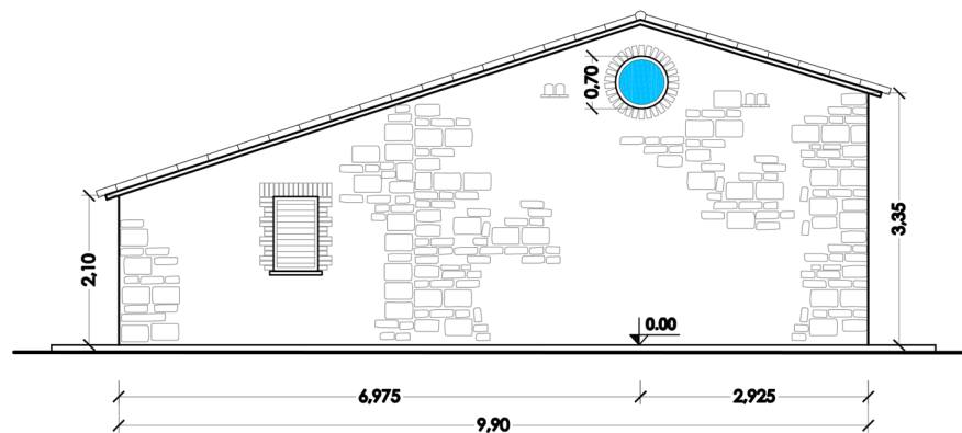
NORTH VIEW Scale 1:100
