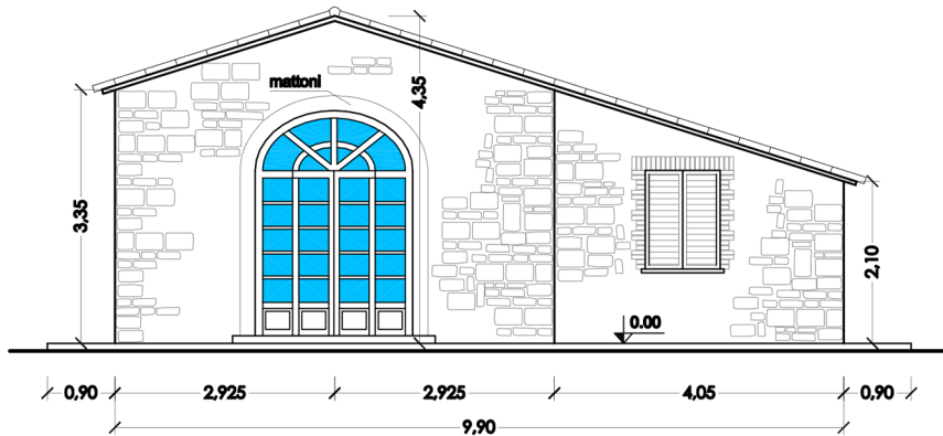
SOUTH VIEW Scale 1:100
