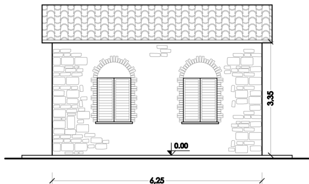
WEST VIEW Scale 1:100
